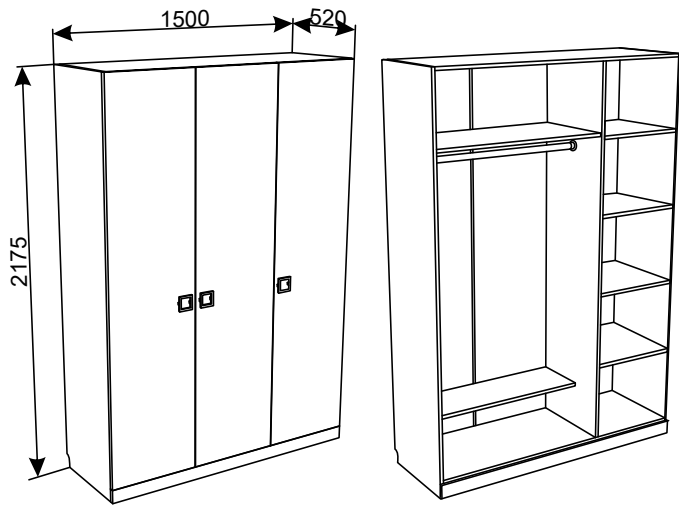
Dulap 3D
